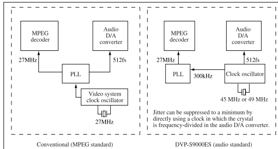
Fig. 19: Contrary to common practice, the DVP-S9000ES subdivides the audio master clock for video, not the other way around.
